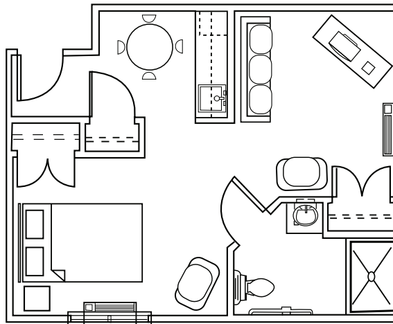
Companion Apartment, (Type 4) – 500 sq. ft.
